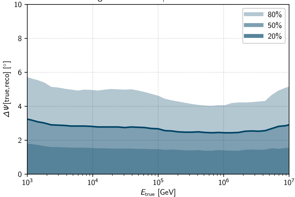
DNN Angular Resolution | True-and-Reco-Tracks
