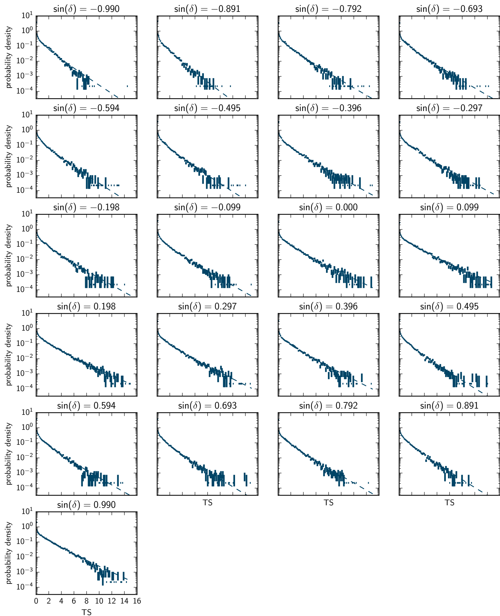
Background-only TS distributions: DNN (loc=0)
