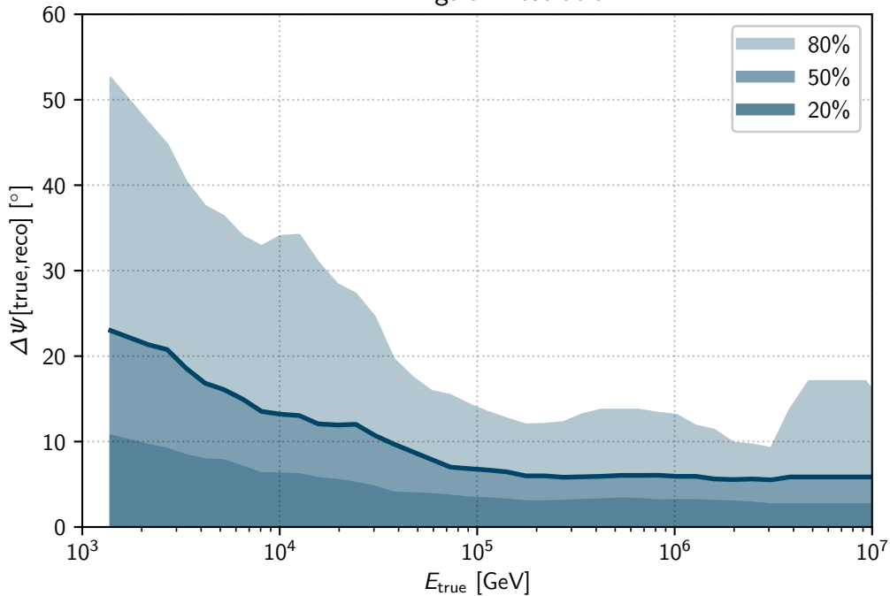
DNN Angular Resolution
